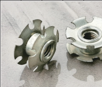
Name:Spring Threaded inserts tube Star Insert Nuts Plum shrapnel nut P/N: JX-SN-M8-D24.5-H12-65Mn Material:Steel+65Mn
