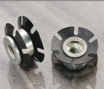
Name:Spring Threaded inserts tube Star Insert Nuts Plum shrapnel nut P/N: JX-SN14-20-24.86-H12.91-65MN Material:Steel+65Mn
