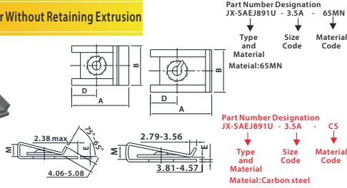
A Type short, B Type Long Material:65MN, Carbon steel, Stainless steel Unit:mm
