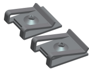
A Type short, B Type Long Material:65MN, Carbon steel, Stainless steel Unit:mm
