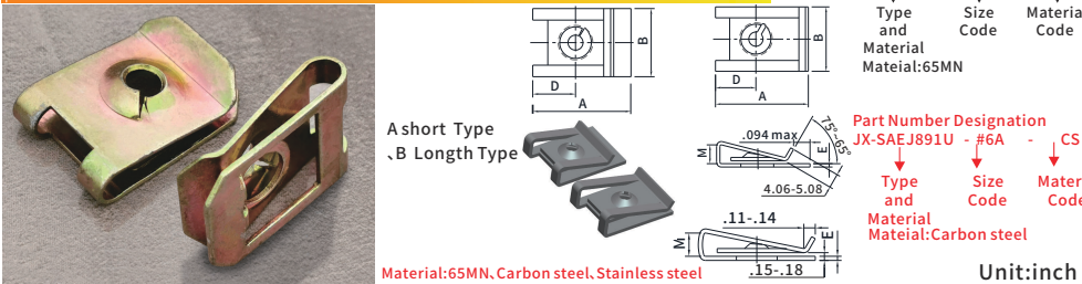
SAE J 891(Figure7)-2016 U Shape Wide-range Design Spring Nuts With Or Without Retaining Extrusion
