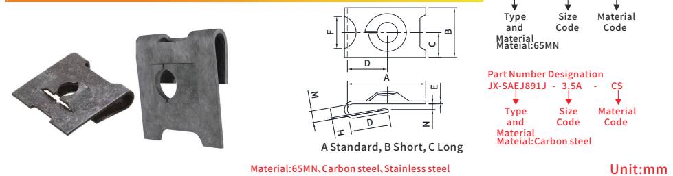
SAE J 891(Figure8)-2016 Type P, J Shape Regular Design Spring Nuts
