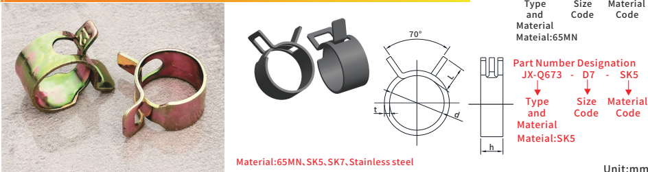
Material:65MN,SK5,SK7,Stainless steel
