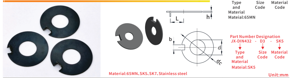
Material:65MN,SK5,SK7,Stainless steel
