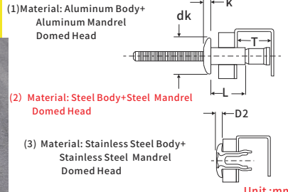
(1)Material: Aluminum Body+ Aluminum Mandrel Domed Head (2) Material: Steel Body+Steel Mandrel Domed Head (3) Material: Stainless Steel Body+ Stainless Steel Mandrel Domed Head
