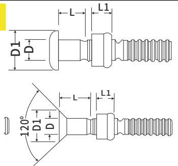
(1)Material: (Aluminum) P/N:JX-D-L-AL (2)Material:(Steel) P/N:JX-D-L-ST (3)Material:(Stainless Steel) P/N:JX-D-L-SS
